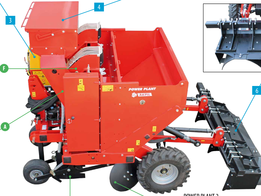
POWER PLANT 2
